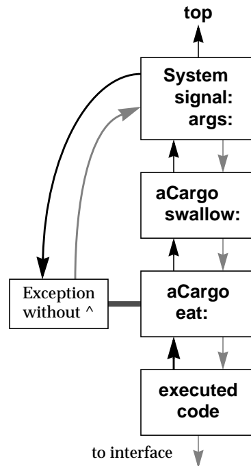
Figure 11.3 Default Flow of Control in Exception-handlers
