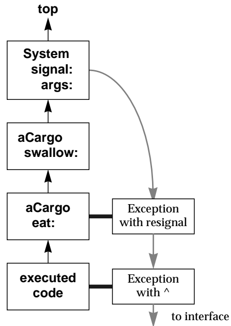
Figure 11.5 Activation Exception-handler Passing Control to Another Handler
